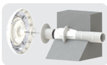
Concrete Pool with Conduit
