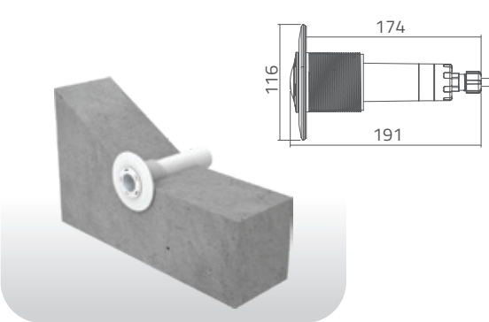
Suction Fittings
