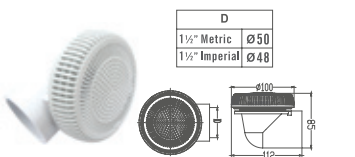
Swirl Type Water Return
