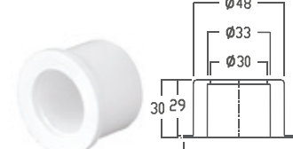
Pipe Plug
