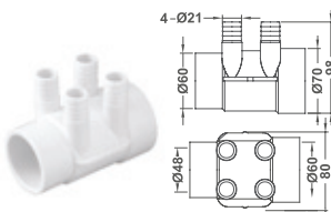
Port Water Barb Manifold
