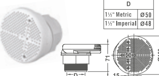
φ2 Section Drain Lock Nut
