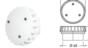
φ2 Section Drain Straight Body(with Bolt)
