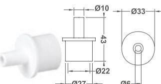
Barb Plug
