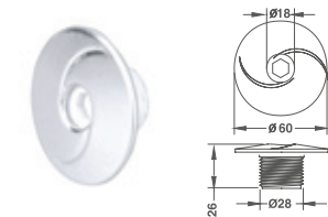
φ2" Face (Spiral) Jet
