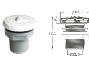
Standard Air Control
