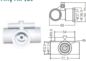
Tiny Air Jet
