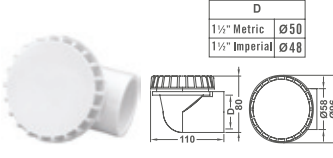
φ2 Section Drain EII Body(Slip Fit)
