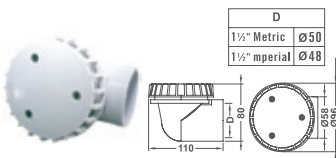
φ2 Section Drain EII Body(Threaded)
