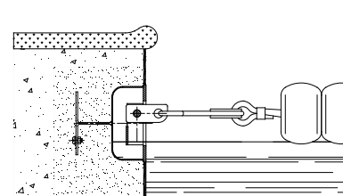
Anchoring cup code 09206 code 09207 code 00205 code 00206
