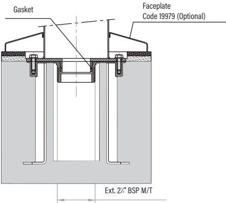
Anchor detail
