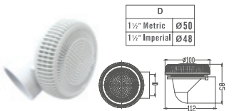
Swirl Type Water Return
