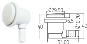
Single Hole Air Jet
