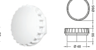
φ2 Section Drain Straight Body
