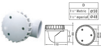
φ2 Section Drain EII Body(Threated)
