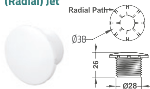
φ1-1/2" Face (Radial) Jet
