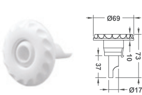
φ2-3/4" Vortex Face Eyeball Spa Jet
