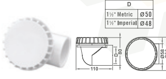
φ2 Section Drain EII Body(Slip Fit)
