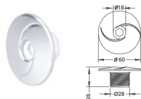
φ2" Face (Spiral) Jet
