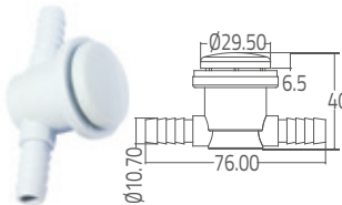
Twin Hole Air Jet
