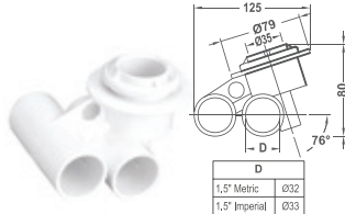
φ25mm Barb Air & φ25mm Water Tee Body
