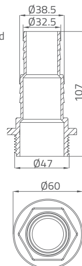
Code: 91609011 Barbed 32/38mm to 1-1/2" Male threaded
