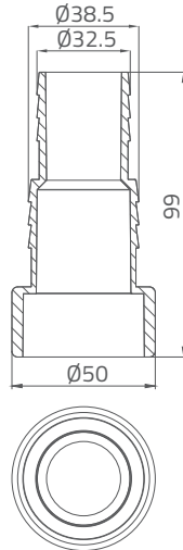
Code: 91609006 Barbed 32/38mm to Solvent 50mm
