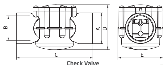
Check Valve
