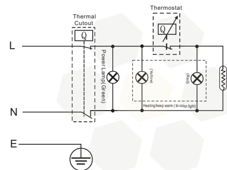
Diagram 7 Wiring diagram
