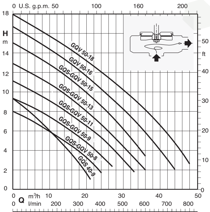
Coverage chart n ≈ 2900 rpm
