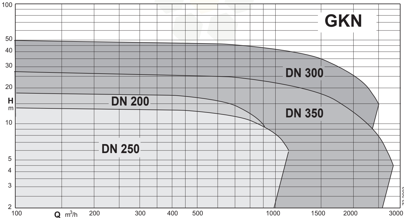
submersible pumps with channels impeller
