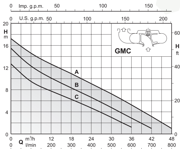
Coverage chart n \approx 2900 rpm
