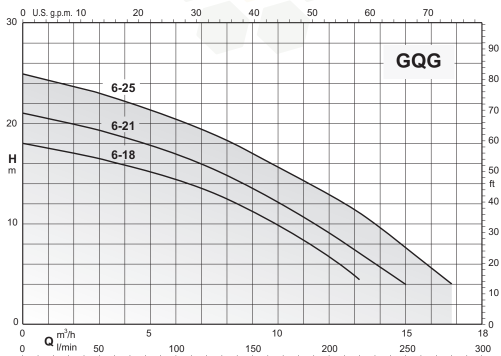
Coverage chart n \approx 2900 rpm
